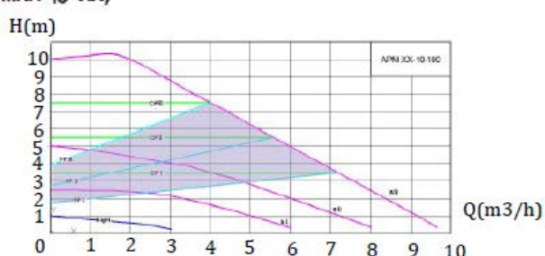
(APMXX -10- XX)
