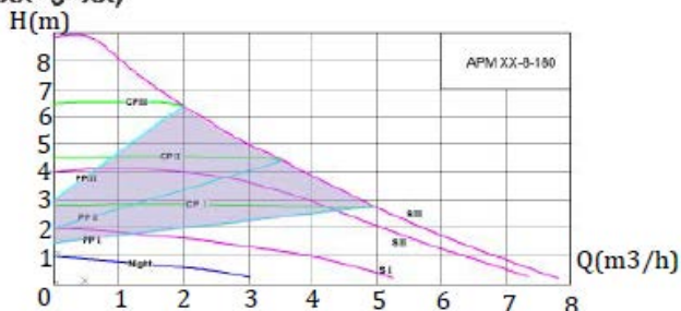
(APMXX -8- XX)
